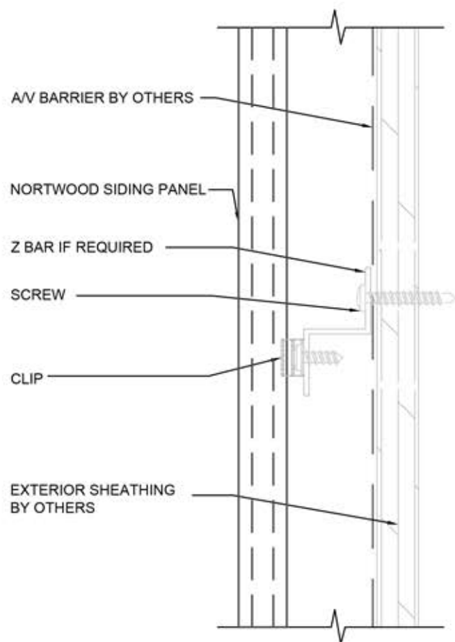
VERTICAL JOINT TYP.
