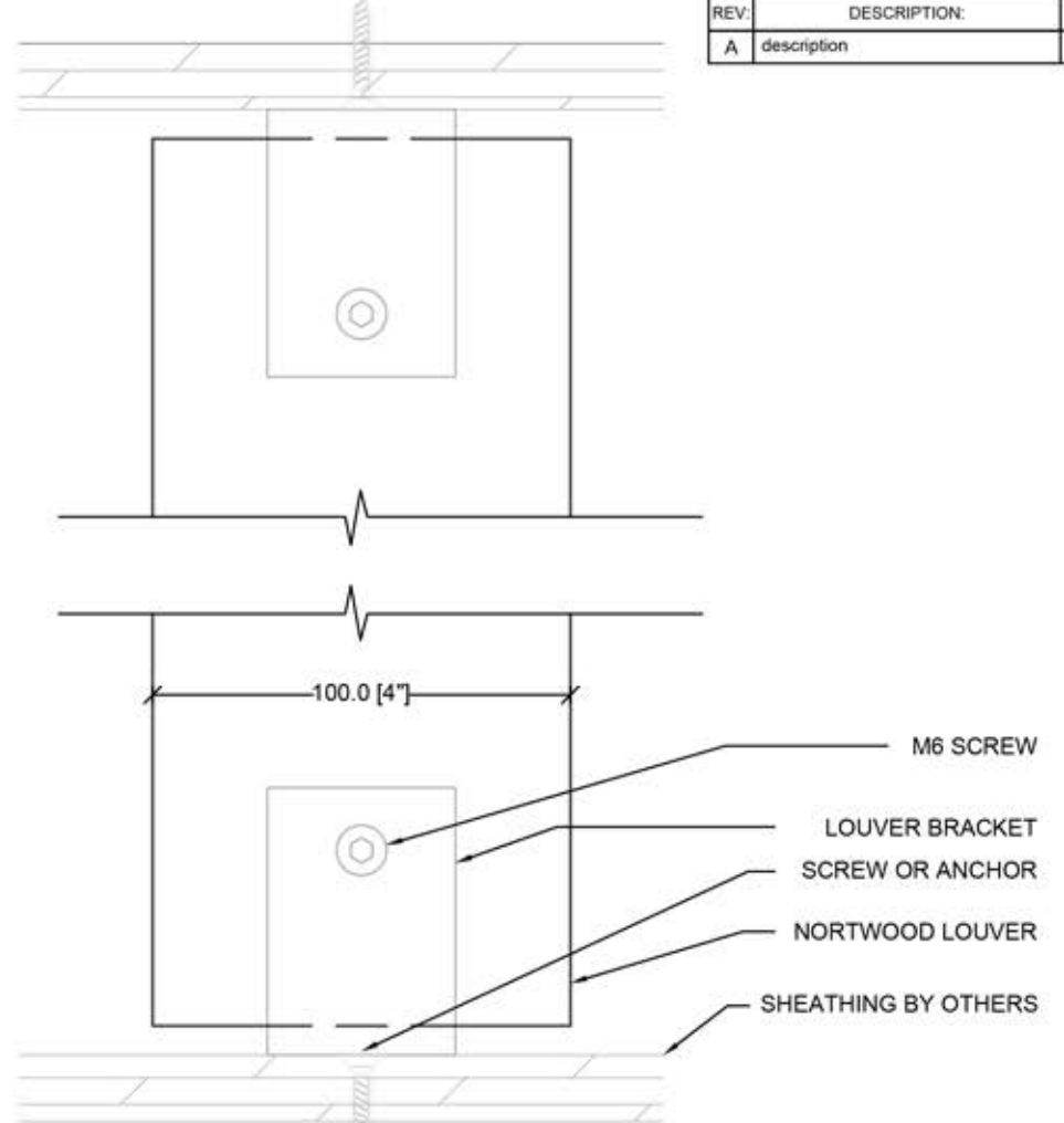
LOUVER ATTACHED FROM SIDE LOUVER ATTACHED TOP/BOTTOM
