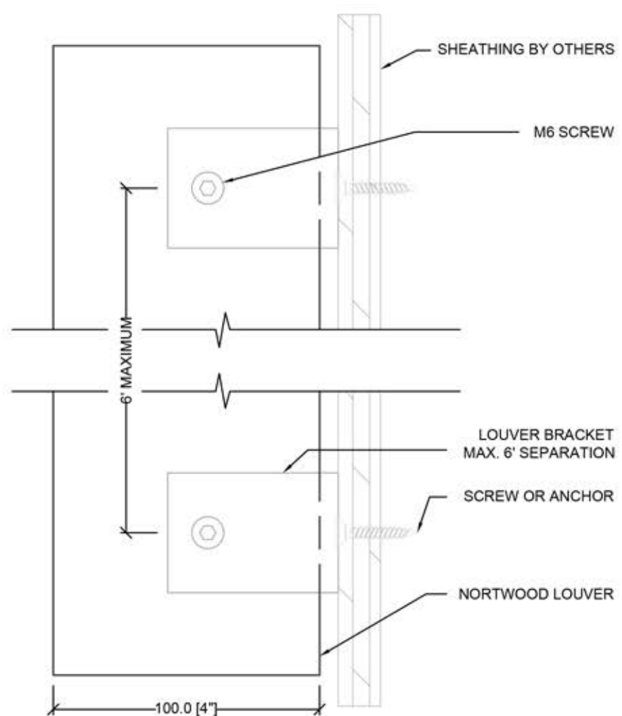
LOUVER ATTACHED FROM SIDE LOUVER ATTACHED TOP/BOTTOM
