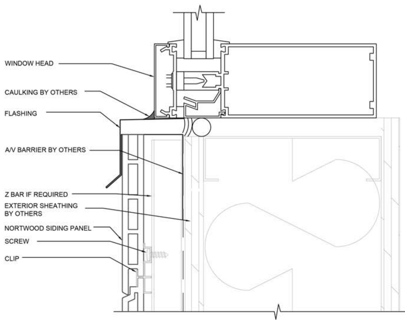
HORIZ. INST. AT WINDOW SILL
