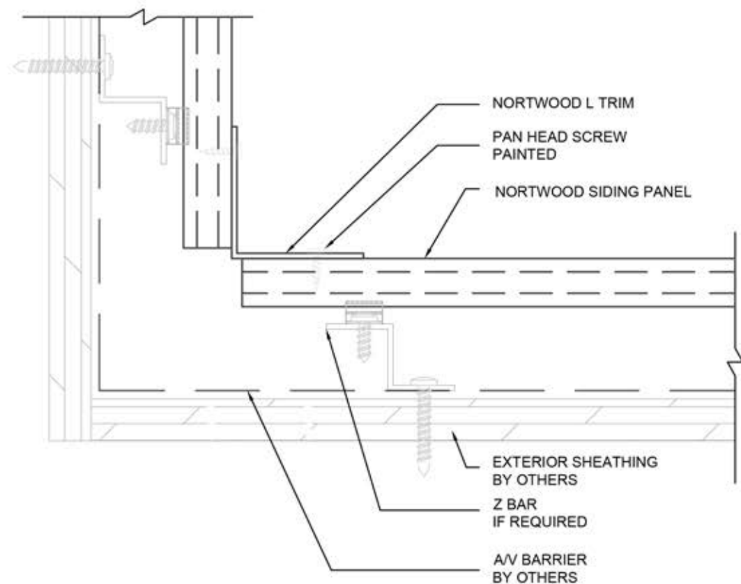
INSIDE CORNER L TRIM
