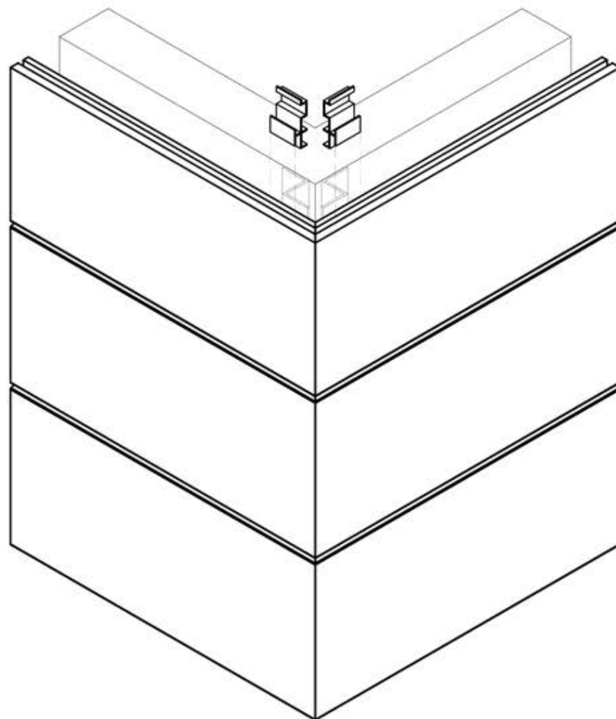
SIDING PANEL
