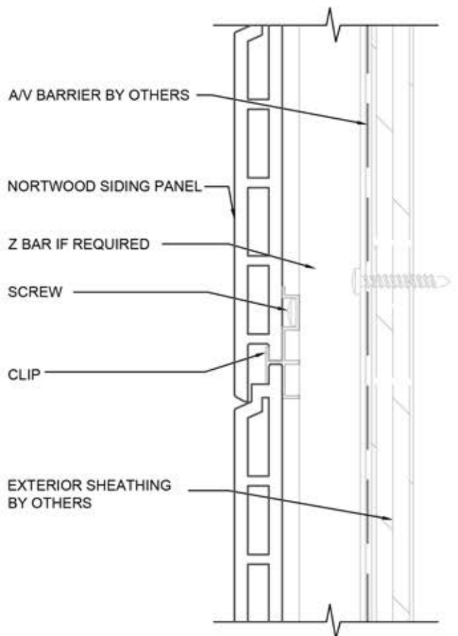
HORIZONTAL JOINT TYP.
