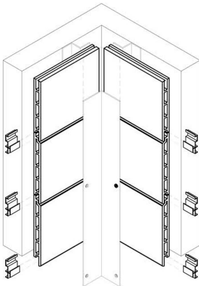
SIDING PANEL
