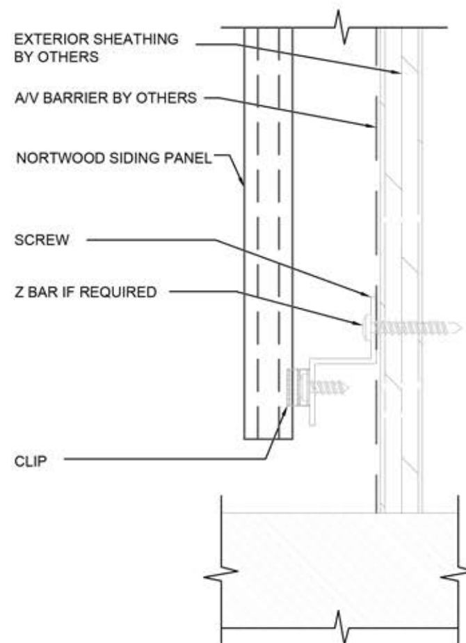
VERTICAL INS. END
