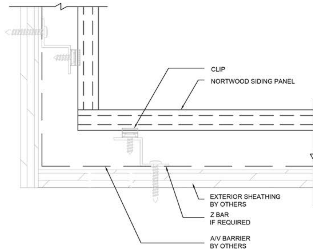
INSIDE CORNER BUTT JOINT
