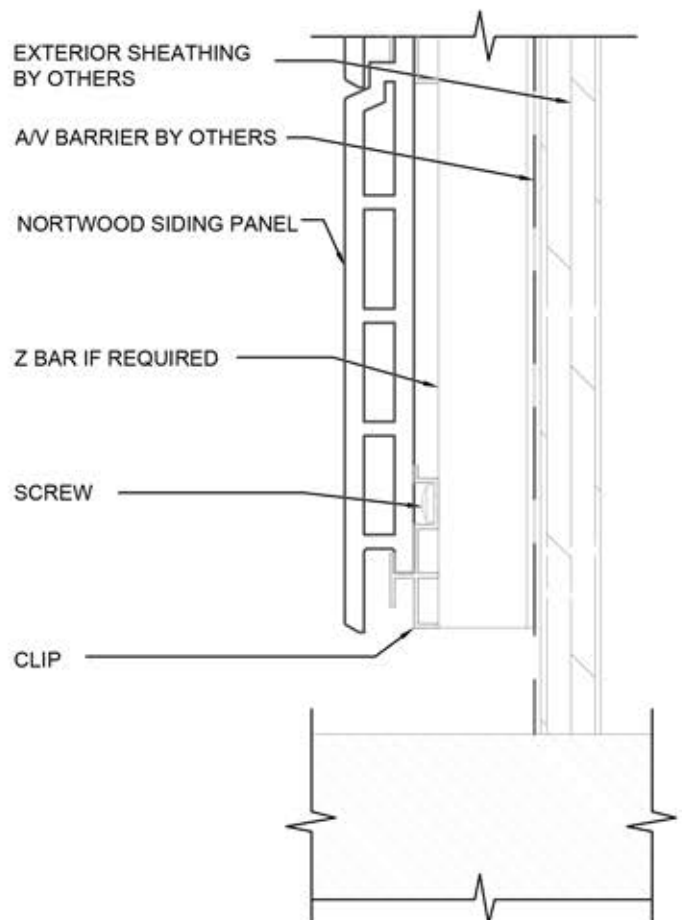
HORIZONTAL INS. END
